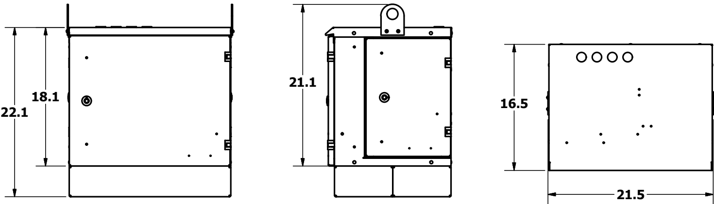
Dimensions are in Inches
